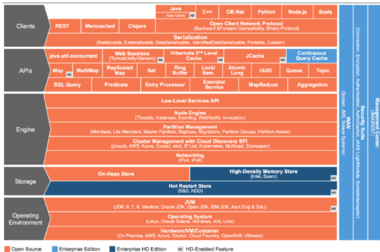
Figure 1.1: Hazelcast Architecture
